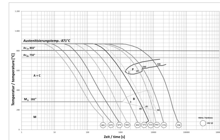
CCT-diagram
